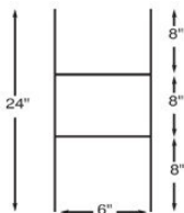
Standard Step Frame
